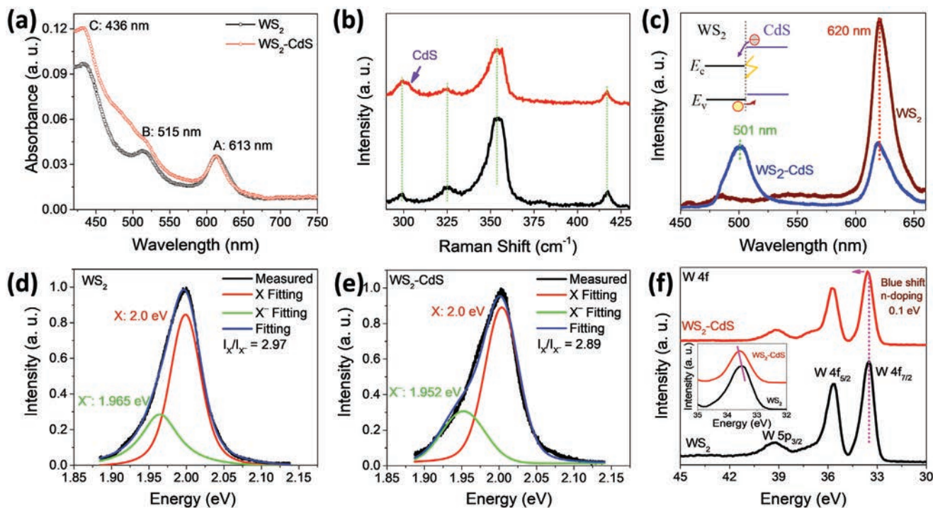
Figure 4. Spectra characterization of the obtained monolayer \text{WS}_2 and \text{WS}_2 -CdS heterostructure. a) Optical absorption spectra. b) Raman spectra excited by a 532 nm laser. The peak associating with CdS is pointed out by a purple arrow. The peaks belonging to \text{WS}_2 are indicated by the dashed green line. c) PL spectrum excited by a 405 nm laser. Inset: Band alignment of the \text{WS}_2 -CdS heterostructure. d,e) PL peak fittings for monolayer \text{WS}_2 and \text{WS}_2 -CdS heterostructure. f) XPS of W 4f peak. Inset: Enlarged part of W 4f_{7/2} peak illustrating the blue-shift of the peak after heterostructure formation.
