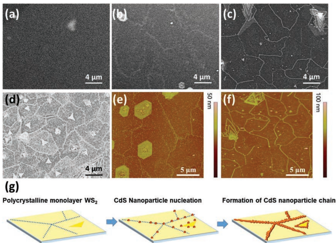
Figure 3. Morphology evolution and proposed mechanistic growth model of the obtained WS 2 -CdS heterostructure. Morphology evolution as a function of the CdS deposition time. a) As prepared, SEM image. b) 4 min, SEM image. c) 10 min, SEM image. d) 60 min, SEM image. e) 4 min, AFM image. f) 10 min, AFM image. g) Schematic illustration of the proposed growth mechanism of CdS on WS 2 . The light and dark yellow areas stand for the single and multilayer WS 2 domains, respectively. The blue dotted lines represent the WS 2 grain boundaries while the brown dots designate the CdS nanomaterials.
