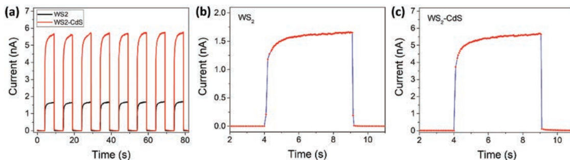
Figure 7. Transient properties of the WS 2 and WS 2 -CdS heterostructure photodetectors. a) Current versus time response under modulated light illumination. Magnified part of the curve of b) WS 2 and c) WS 2 -CdS heterostructure based photodetectors. The light intensity and bias voltage is 4.9 mW cm -2 and 4 V, respectively.
